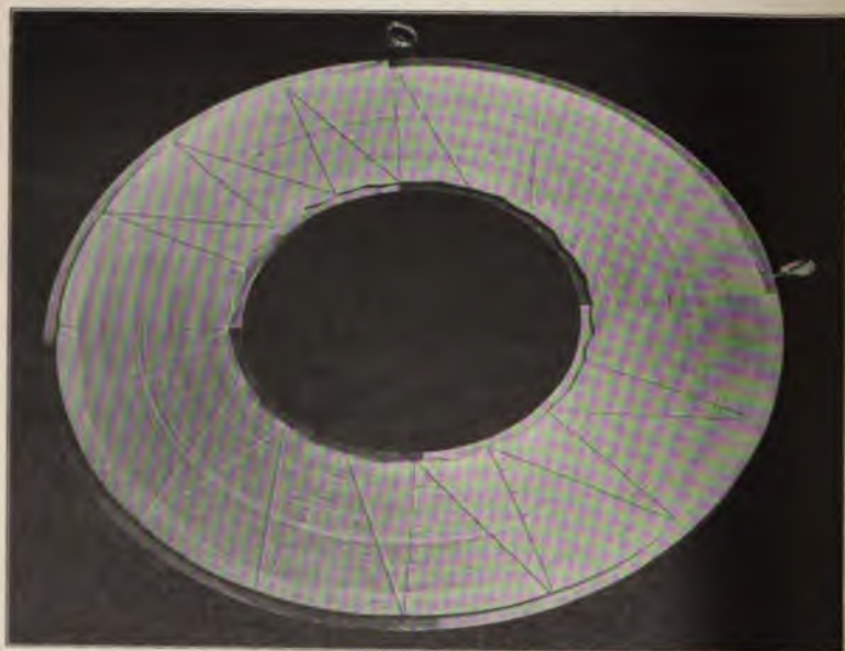
FIG. 2.— COIL OF 200,000-VOLT TRANSFORMER, 1904.
